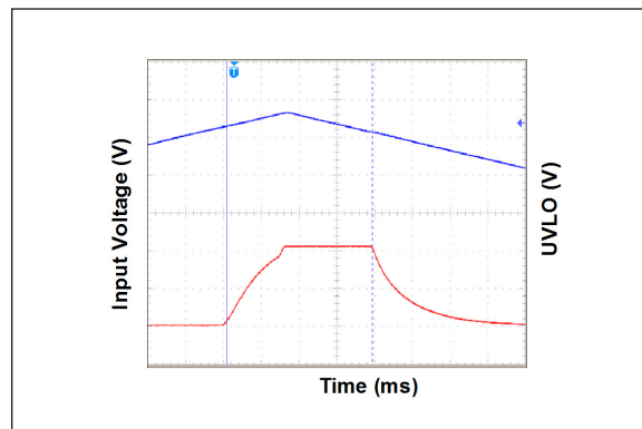
FIGURE 2-24: Undervoltage Lockout.
