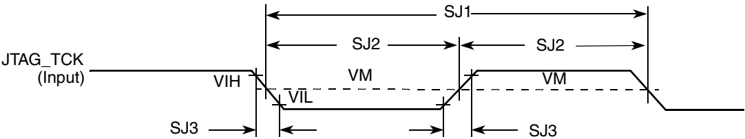
Figure 59. Test Clock Input Timing Diagram
