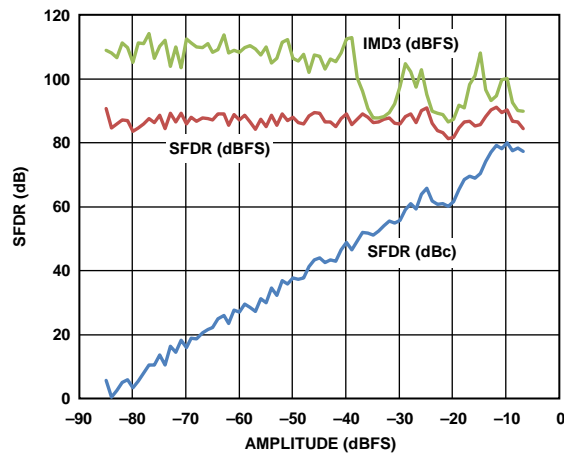
Figure 17. Two Tone SFDR and IMD3 vs. Analog Input Amplitude at 2.0 GSPS at 1800 MHz AIN
