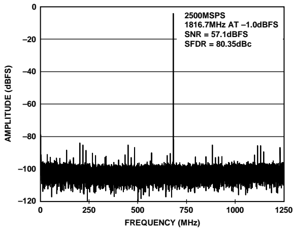
Figure 6. FFT Plot at 2.5 GSps, f_{IN} = 1816.7 MHz at AIN (SFDR = 80.4 dBc, SNR = 57.1 dBFS)
