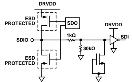
Figure 53. Equivalent SDIO Circuit
