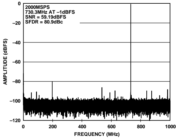
Figure 13. FFT Plot at 2.0 GSPS, f_{IN} = 730.3 MHz at AIN (SFDR = 80.9 dBc, SNR = 59.2 dBFS)
