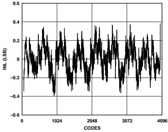
Figure 42. Integral Nonlinearity (INL), \pm 0.4 LSB at 2.0 GSPS
