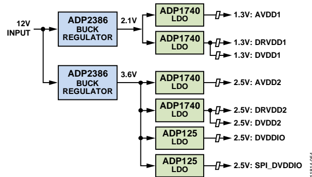
Figure 86. Power Supply Recommendation
