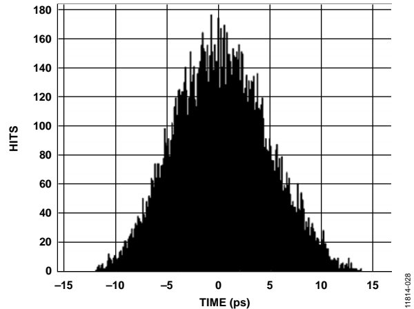
Figure 73. Time Interval Histogram Error of JESD204B Output at 6.25 Gbps
