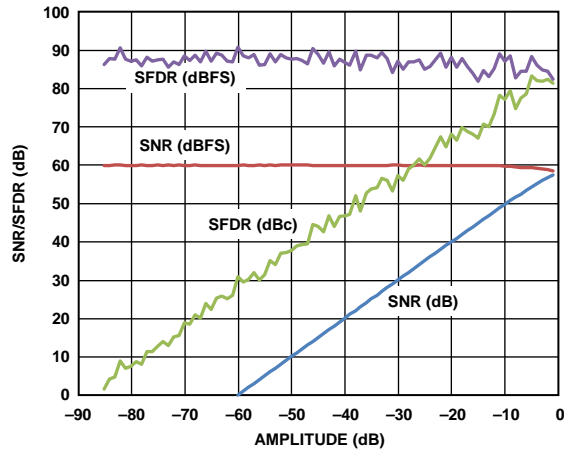
Figure 16. SNR/SFDR vs. Analog Input Amplitude at 2 GSPS, f_{IN} = 1811.3 MHz at AIN
