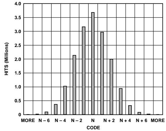
Figure 33. Input Referred Noise Histogram with 2.5 GHz Sample Clock
