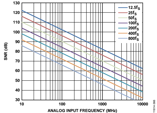
Figure 61. Ideal SNR vs. Analog Input Frequency and Jitter
