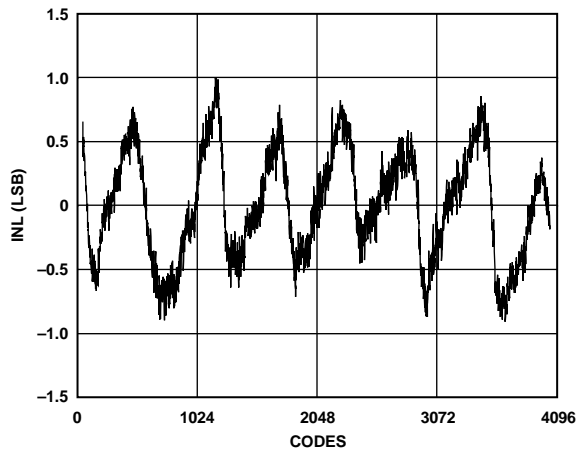
Figure 43. Integral Nonlinearity (INL), \pm 1.0 LSB at 2.5 GSPS
