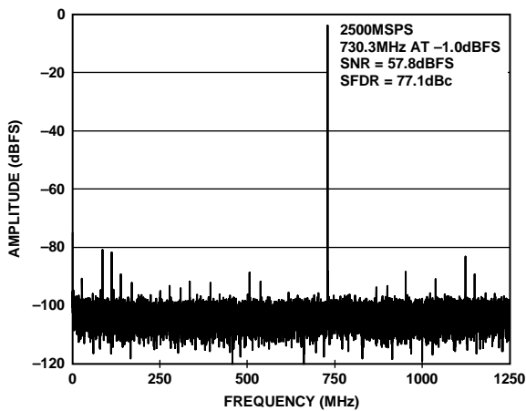
Figure 7. FFT Plot at 2.5 GSps, f_{IN} = 730.3 MHz at AIN (SFDR = 77.8 dBc, SNR = 57.8 dBFS)
