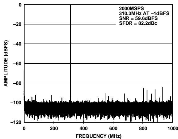
Figure 14. FFT Plot at 2.0 GSPS, f_{IN} = 310.3 MHz at AIN (SFDR = 82.2 dBc, SNR = 59.6 dBFS)
