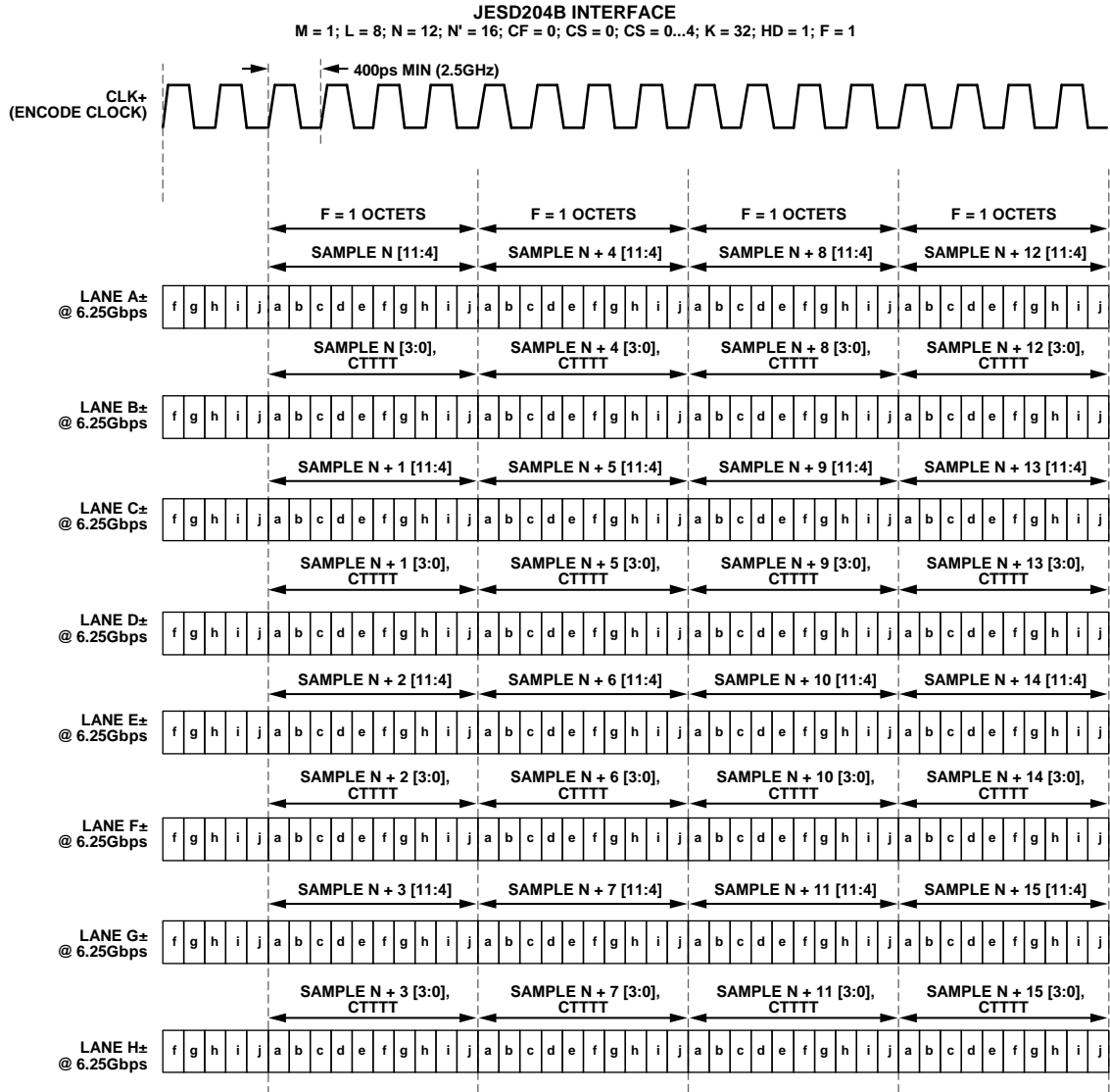
Figure 68. JESD204B Lane Data Mapping
