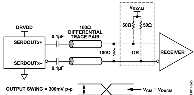
Figure 69. AC-Coupled Digital Output Termination Example
