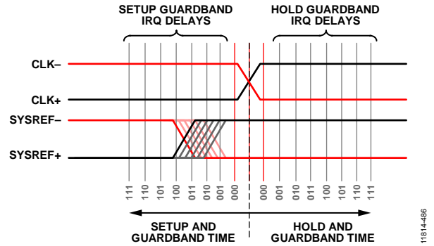
Figure 81. SYSREF \pm Edge Changes Phase Relative to the Encode Clock, Which can be Detected When the Edge Crosses Through the Guardband Setup Time
