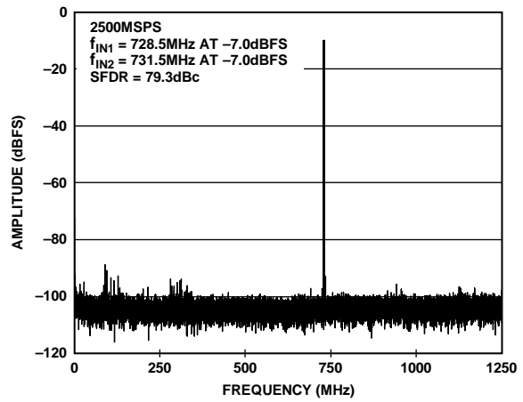
Figure 35. Two Tone FFT Plot at 2.5 GSPS, f_{IN1} = 728.5 MHz and f_{IN2} = 731.5 MHz at AIN, -7 dBFS (SFDR = 79 dBc)
