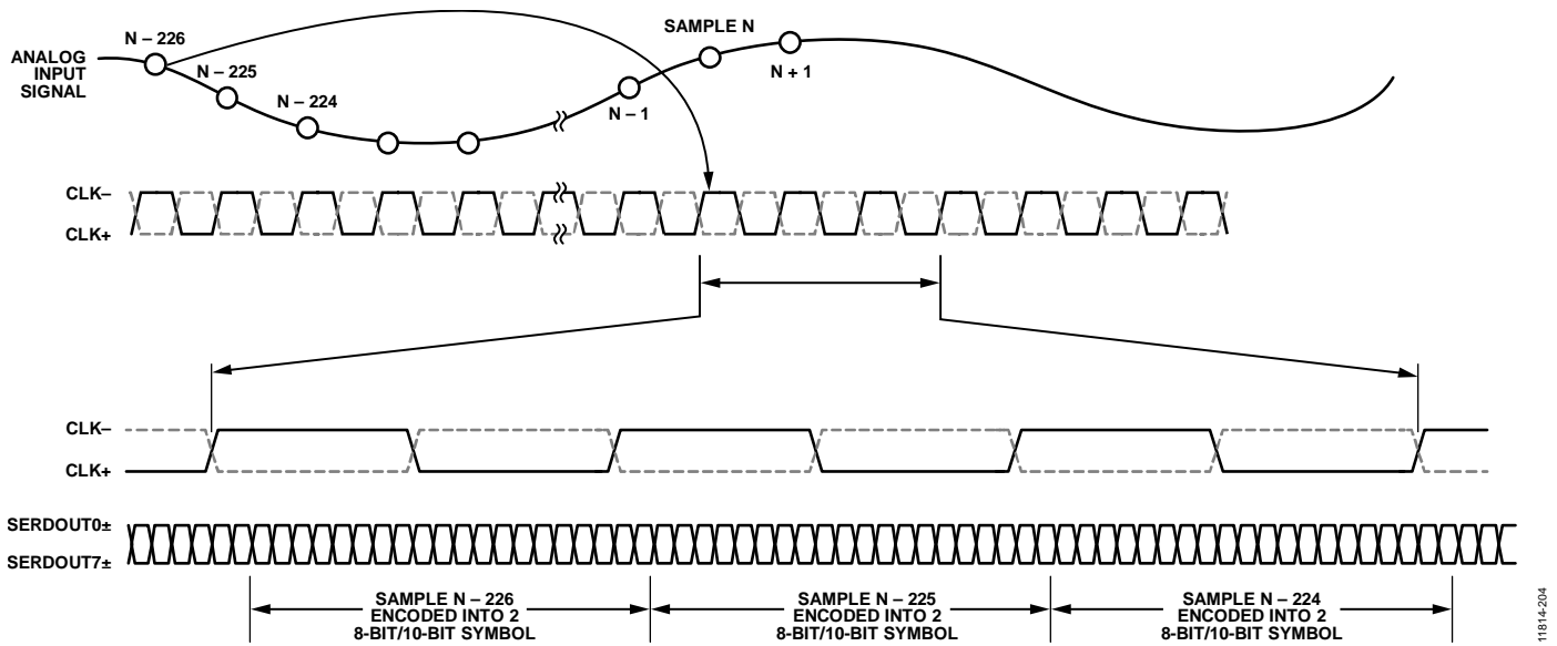
Figure 4. Data Output Timing for 8 Lane Mode
