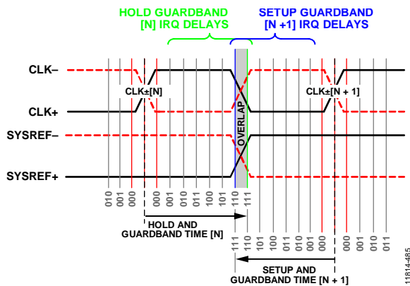
Figure 80. SYSREF \pm Edge Falls Within Both the Latest Hold Time Guardbanded of CLK \pm [N] and the Earliest Setup Time Guardband of CLK \pm [N + 1] and Triggers an IRQ Error
