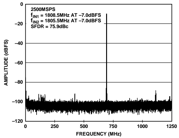
Figure 34. Two Tone FFT Plot at 2.5 GSPS, f_{IN1} = 1808.5 MHz and f_{IN2} = 1805.5 MHz at AIN, -7 dBFS (SFDR = 76 dBc)
