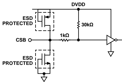
Figure 49. Equivalent CSB/PWDN Input Circuit
