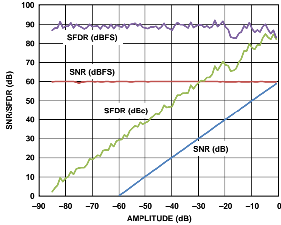
Figure 15. SNR/SFDR vs. Analog Input Amplitude at 2 GSPS, f_{IN} = 241.1 MHz at AIN
