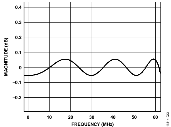
Figure 66. Magnitude Ripple in the Low Bandwidth Pass Band
