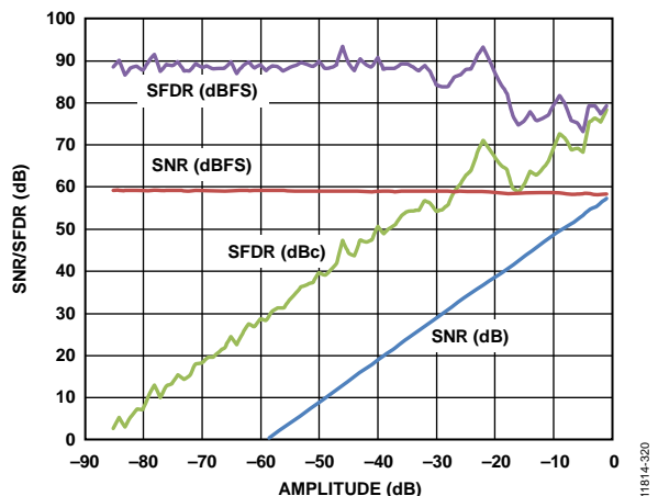
Figure 20. SNR/SFDR vs. Analog Input Amplitude at 2.5 GSPS, f_{IN} = 241 MHz at AIN
