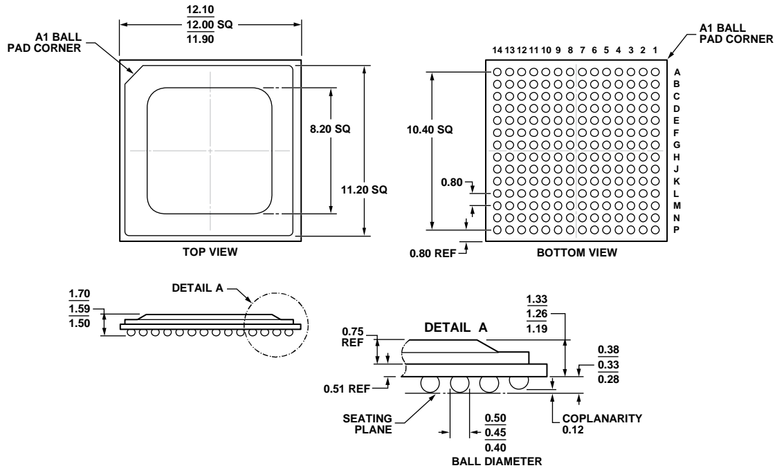
Figure 87. 196-Ball Ball Grid Array, Thermally Enhanced [BGA_ED] (BP-196-2)
