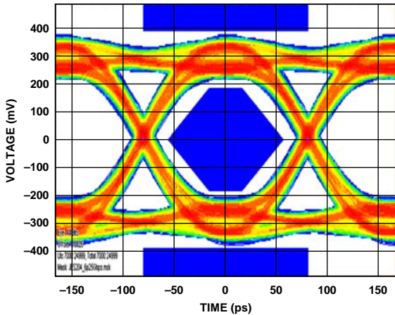
Figure 71. Recovered Data Eye of JESD204B Lane at 6.25 Gbps
