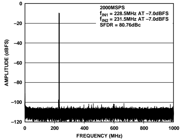
Figure 39. Two Tone FFT Plot at 2.0 GSps, f_{IN1} = 228.5 MHz and f_{IN2} = 231.5 MHz at AIN, -7 dBFS (SFDR = 81 dBc)
