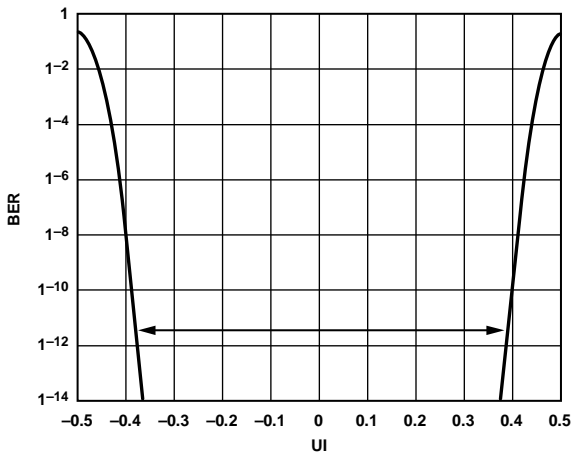
Figure 72. Bathtub Plot of JESD204B Output at 6.25 Gbps
