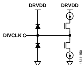
Figure 50. Equivalent DIVCLK Output Circuit (DRVDD)
