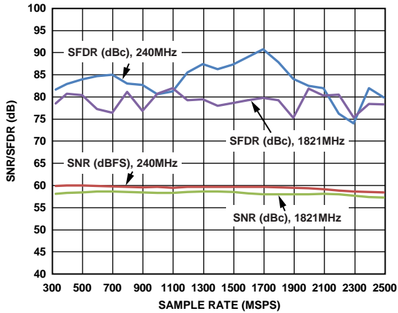
Figure 30. SNR/SFDR vs. Sample Rate
