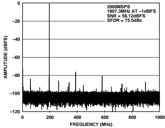
Figure 12. FFT Plot at 2.0 GSPS, f_{IN} = 1807.3 MHz at AIN (SFDR = 75.5 dBc, SNR = 58.1 dBFS)
