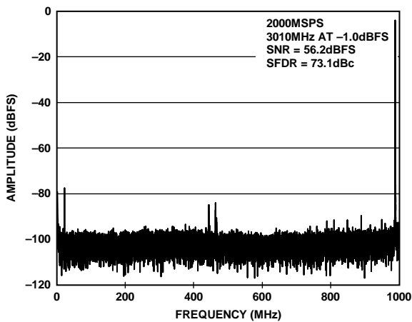
Figure 8. FFT Plot at 2.0 GSps, f_{IN} = 3010 MHz at AIN (SFDR = 73 dBc, SNR = 56 dBFS) (Input Network in Figure 60 Used)
