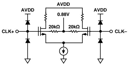
Figure 48. Equivalent Clock Input Circuit
