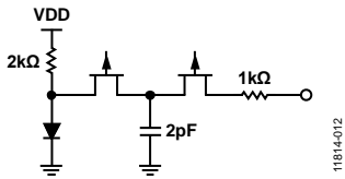
Figure 47. Equivalent VMON Temperature Sensor Circuit (DVDD)
