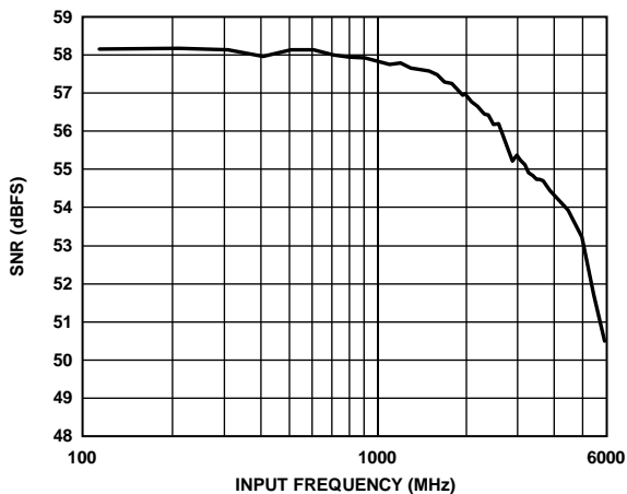
Figure 32. SNRFS vs. AIN Frequency at 2.5 GSPS (Input Network in Figure 60 Used <2 GHz, Input Network in Figure 59 Used >2 GHz)
