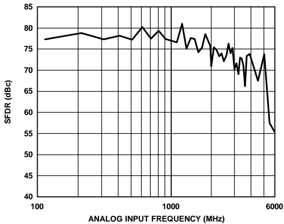
Figure 31. SFDR vs. AIN frequency at 2.5 GSPS (Input Network in Figure 60 Used <2 GHz, Input Network in Figure 59 used >2 GHz)
