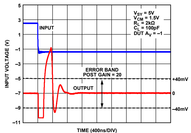
Figure 51. Negative Setting Time to 0.1%, V_{SY} = 5\text{ V}
