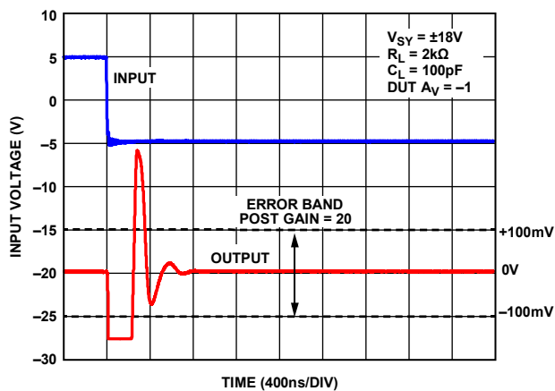
Figure 48. Negative Setting Time to 0.1%, V_{SY} = \pm 18\text{ V}
