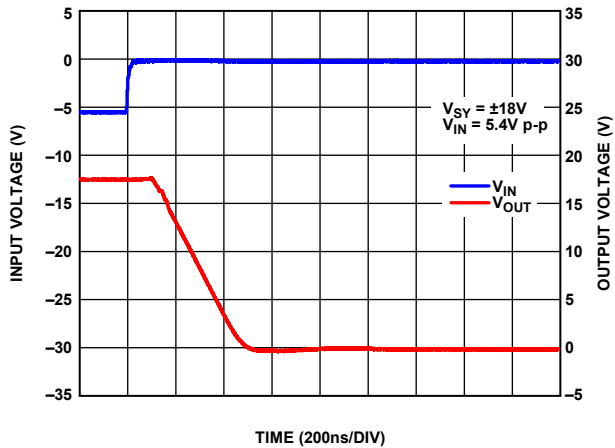
Figure 47. Positive Overload Recovery, A_V = -10 , V_{SY} = \pm 18\text{ V}
