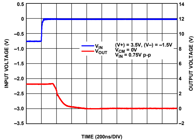
Figure 50. Positive Overload Recovery, A_V = -10 , V_{SY} = 5\text{ V}
