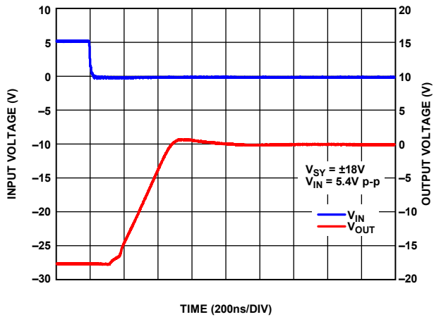
Figure 46. Negative Overload Recovery, A_V = -10 , V_{SY} = \pm 18\text{ V}
