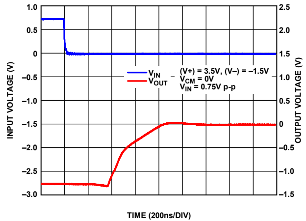
Figure 49. Negative Overload Recovery, A_V = -10 , V_{SY} = 5\text{ V}
