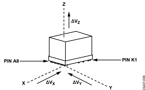
Figure 36. Delta Velocity Axis and Polarity Assignments
