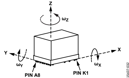
Figure 30. Gyroscope Axis and Polarity Assignments
