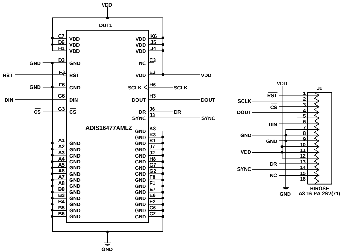
Figure 47. Breakout Board Schematic
