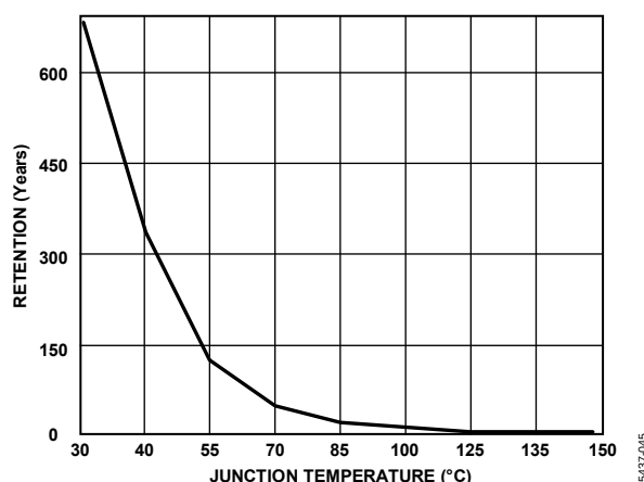
Figure 43. Flash Memory Retention
