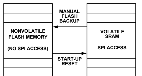
Figure 29. SRAM and Flash Memory Diagram
