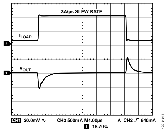
Figure 14. Load Transient Response, C_{\text{OUT}} = 10\text{ }\mu\text{F} , V_{\text{IN}} = 1.7\text{ V} , V_{\text{OUT}} = 1.3\text{ V}
