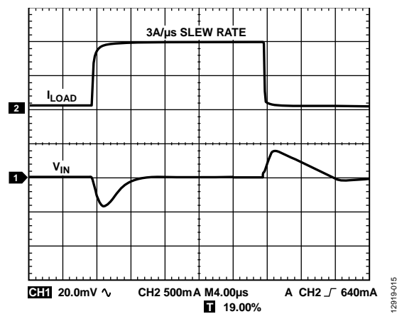
Figure 15. Load Transient Response, C_{\text{OUT}} = 47\text{ }\mu\text{F} , V_{\text{IN}} = 1.7\text{ V} , V_{\text{OUT}} = 1.3\text{ V}
