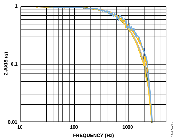
Figure 12. ADXL355 Normalized Frequency Response for Z-Axis at 4 kHz ODR
