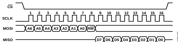
Figure 64. SPI Timing Diagram—Single-Byte Read
