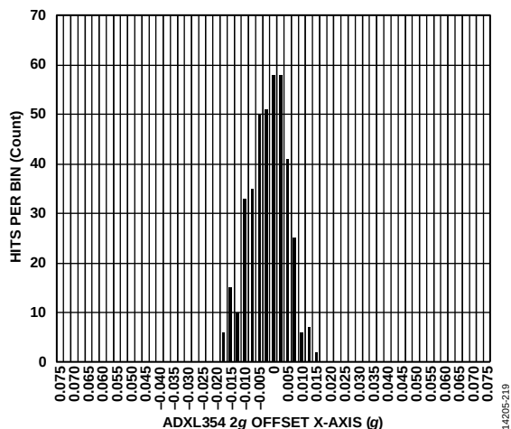
Figure 19. ADXL354 Zero g Offset Histogram at 25°C, X-Axis
