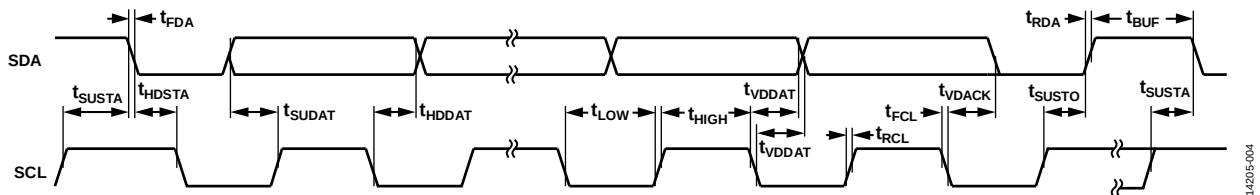
Figure 4. I²C Interface Timing Diagram
