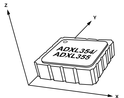
Figure 58. Axes of Acceleration Sensitivity
