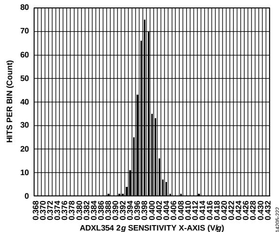
Figure 22. ADXL354 Sensitivity Histogram at 25°C, X-Axis
