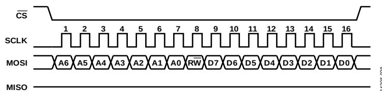
Figure 65. SPI Timing Diagram—Single-Byte Write
